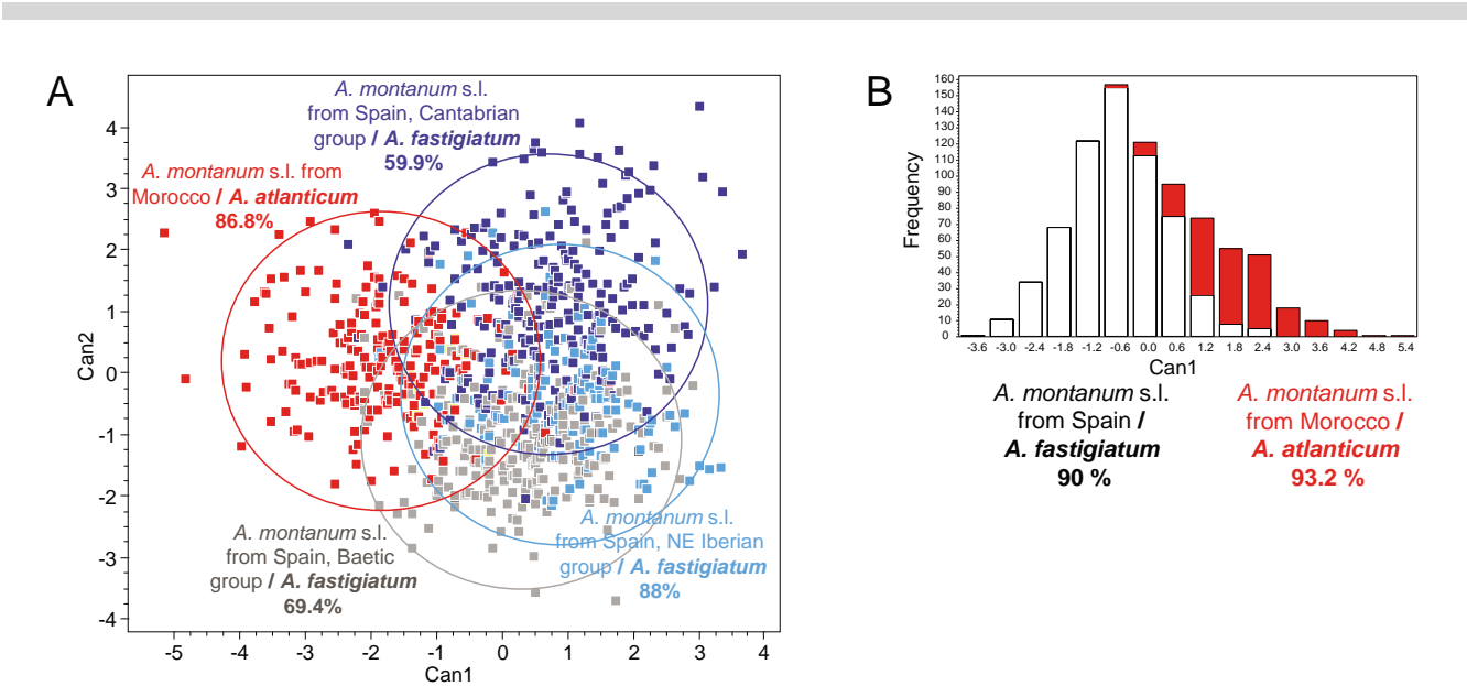
Fig. 8. Discriminant analyses performed on the Spanish and Moroccan populations of A. montanum s.l. ( A. fastigiatum and A. atlanticum in the final treatment, respectively), based on individual plants and 20 morphological characters. The results of the canonical discriminant analyses (CDA) are depicted graphically, while the results of the classificatory discriminant analyses (classificatory DA) are presented as percentage values. The initial taxonomic assignment/final taxonomic treatment (separated by a slash) is given. For total canonical structure, see Table 4. A , CDA 2 and the respective classificatory DA 2 ( k = 21 ) with four predefined groups: Cantabrian (242 plants), NE Iberian (150 plants) and Baetic group of A. fastigiatum (206 plants, excl. populations from Sierra de Mijas), and A. atlanticum from Morocco (205 plants). The 95% isodensity circles are depicted. B , CDA 3 and the respective classificatory DA 3 ( k = 13 ) with two predefined groups: A. fastigiatum (618 plants) and A. atlanticum (205 plants).
