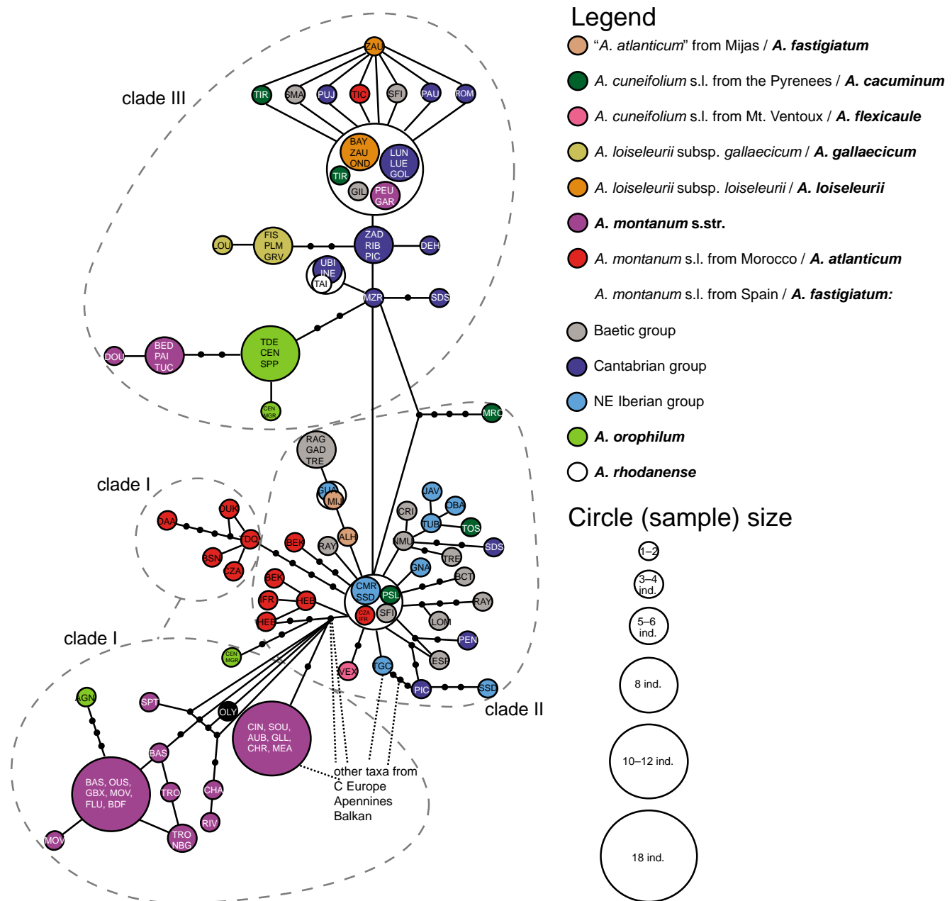
Fig. 6. Maximum parsimony network of the cpDNA (concatenated rpoB-trnC and rpl32-trnL (UAG) alignments) haplotypes of the studied southwestern European and Moroccan Alyssum species. Haplotypes of the taxa from Central Europe and the Balkan and Apennine Peninsulas are not shown, but their positions within the network are indicated (see dotted lines). Circle sizes are proportional to haplotype frequencies (see scale), lines represent mutational steps, and black dots are not sampled haplotypes. Outlines shown in dashed lines encompass the three haplotype groups (I, II and III) as suggested by the Bayesian tree (Electr. Suppl. 1: Fig. S1). Colours indicate species or group affiliation, and both the initial taxonomic assignment and final taxonomic treatment (if different, separated by a slash) are given. Population codes follow Table 1.
