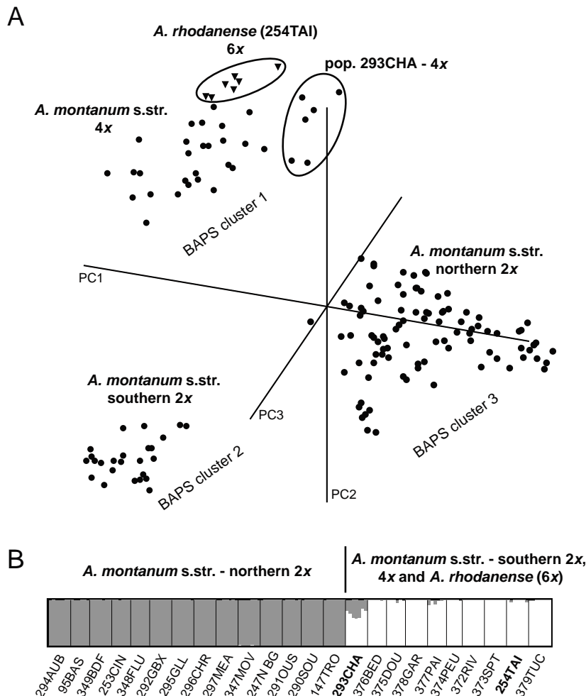
Fig. 5. Genetic structure of A. montanum s.str. and A. rhodanense (159 individuals from 24 populations) based on the AFLP data. A. Principal coordinate analysis based on Jaccard's pairwise genetic distances between individuals. The first three axes explain 10.40%, 6.94% and 5.80% of the variation. The three geographic/cytotype groupings corresponding to the three clusters as also revealed by the BAPS Bayesian clustering are highlighted: southern diploids, northern diploids, and polyploids (tetraploid A. montanum s.str. and hexaploid A. rhodanense ). B. Bayesian model-based clustering (STRUCTURE program) at K = 2 . For the figure description see legend of Fig. 4C. White, southern diploids and polyploids; grey, northern diploids. Population codes follow Table 1.
