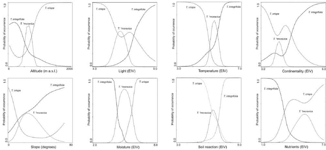
Fig. 5. Species response curves with respect to altitude, slope and six environmental factors expressed by the EIV. Logistic regression fitted by GAM (3 d.f.) were used on the presence/absence data.
