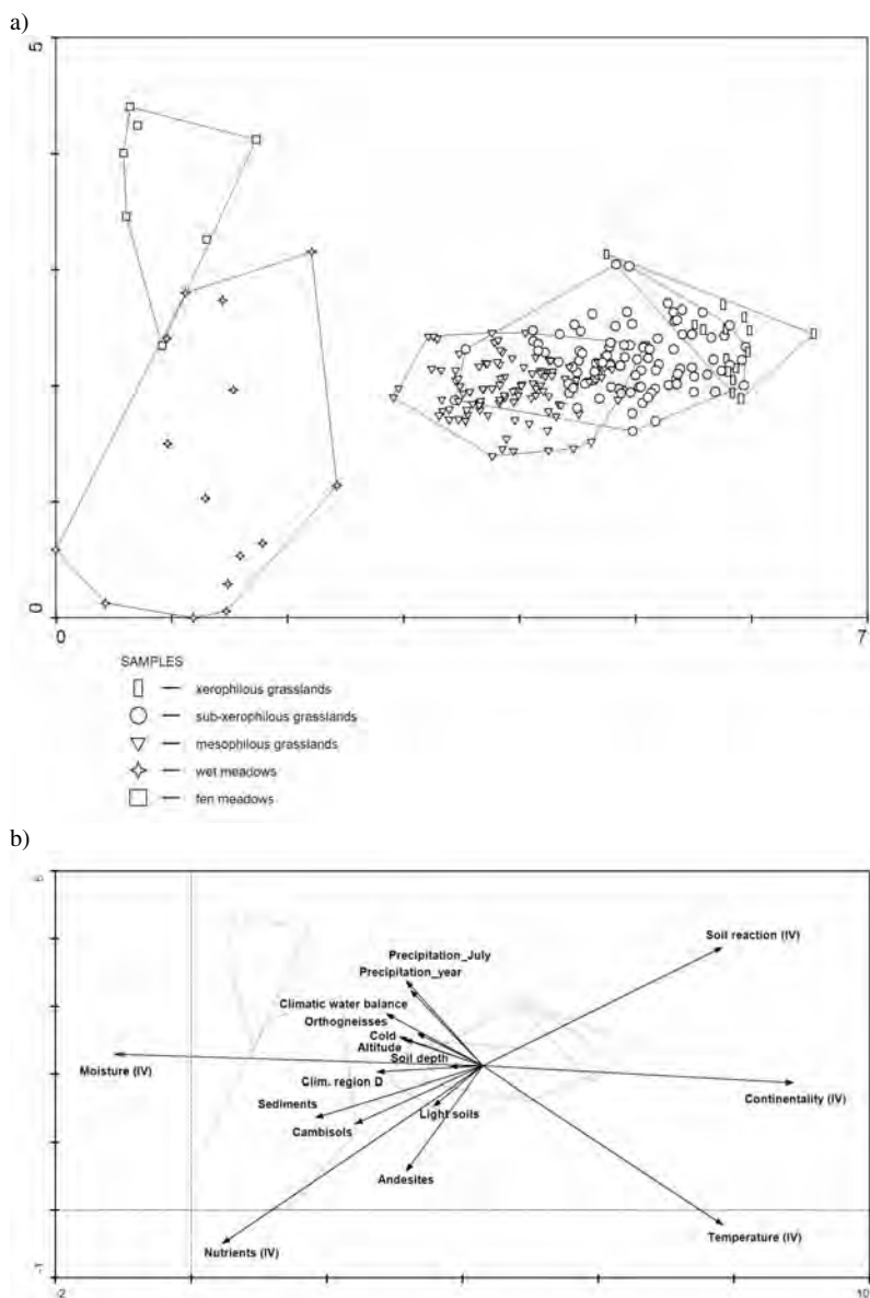
Fig. 3: DCA of the complete data set (eigenvalues: I. axis 0.691, II. axis 0.333; length of gradient of the main ordination axis is 6.5). Relevé positions (a) and supplementary environmental variables with the highest correlation to the ordination axes (b). Wet and fen meadow communities are conspicuously separated from other grassland types along the first ordination axis, which can be interpreted as a moisture gradient ( post-hoc correlation with moisture IV was -0.98 ). The second axis represents the nutritional status of habitats ( post-hoc correlation with nutrients IV was -0.48 ).
