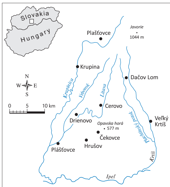
Figure 1: Study sites.
